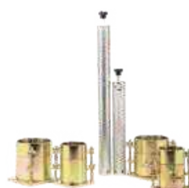
Proctor Compaction Apparatus
